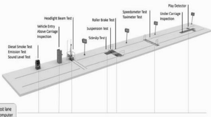
Light / medium vehicles
